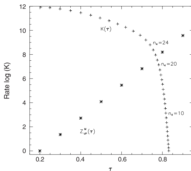
Fig. 3. Relative nonradiative rate (Eq. (1)) K = k_{\text{nr}}(E_{\text{ex}})/k_{\text{nr}}(E_{\text{ex}} = 0) of the \nu_4 progressions (crosses) and Z_{\text{VP}}^{\text{M}}(\tau) (Eq. (6)) (stares) as function of the correlation parameter (saddle-point parameter) \tau .
